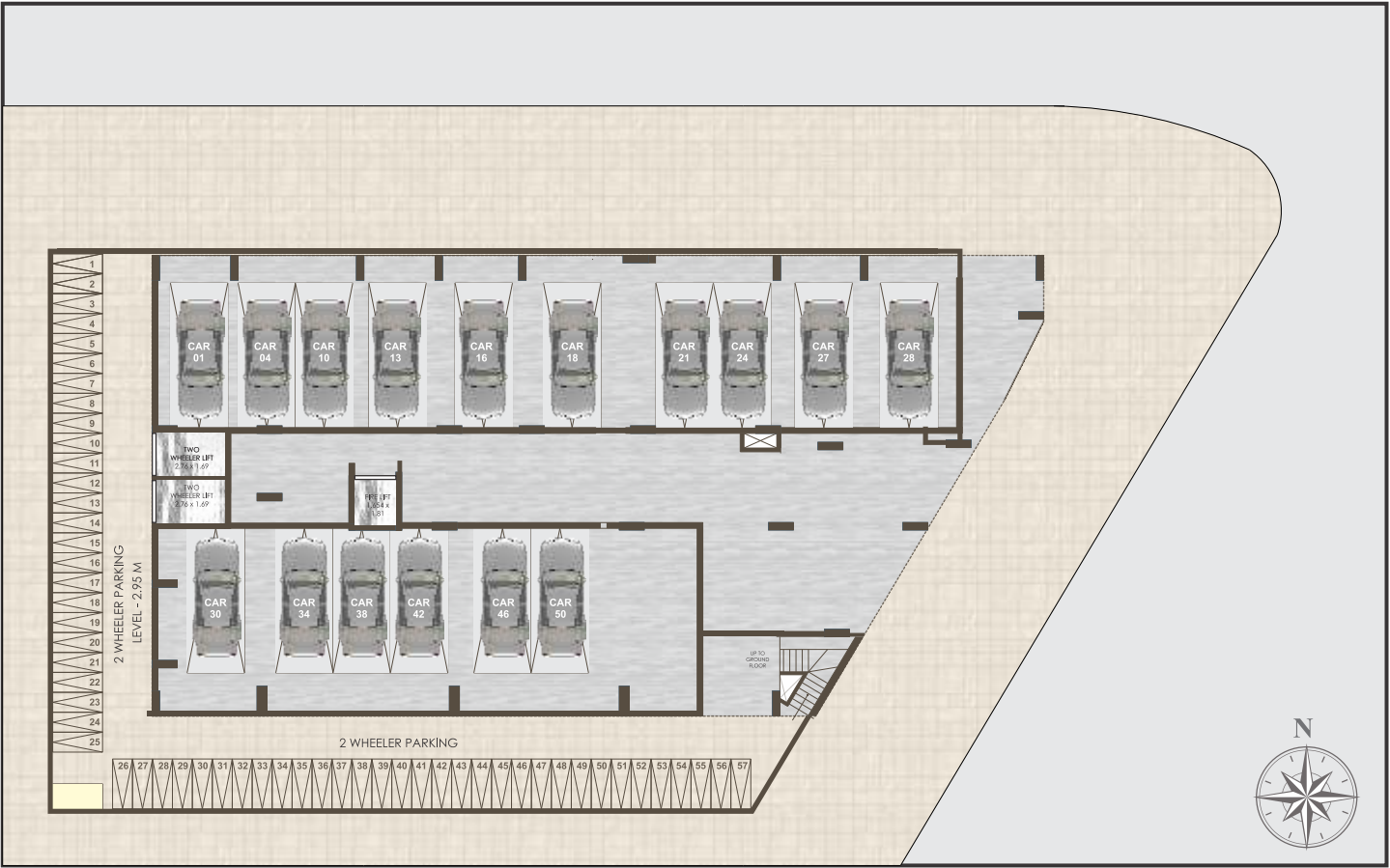
PIT - LEVEL I PLAN ( TWO & FOUR WHEELER PARKING)
